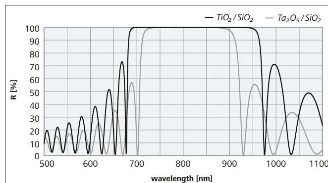
Figure 4: Reflectance spectra of quarter-wave stacks consisting of 15 pairs of \text{Ta}_2\text{O}_5/\text{SiO}_2 and \text{TiO}_2/\text{SiO}_2
