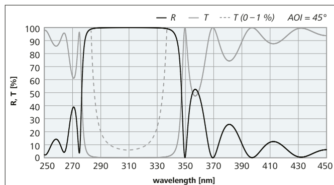
Figure 7: Transmittance spectrum of a sputtered attenuator (IBS) for 308 nm with exactly adjusted and thermally stable transmittance of T = 0.08\% at \text{AOI} = 45^\circ (unpolarized light)
