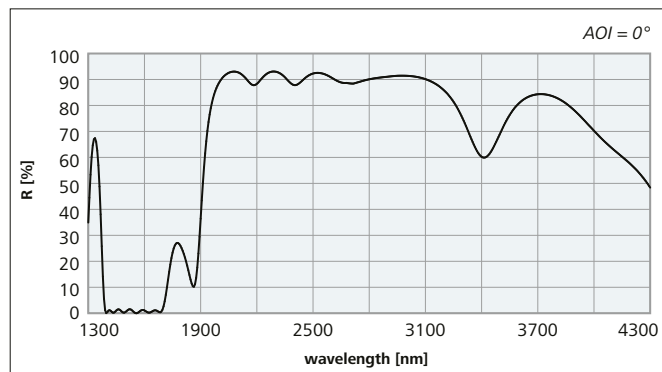
Figure 9: Reflectance spectrum of a special output coupler: PR (0°, 2000 – 3150 nm) = 90 % \pm 3 % + R (0°, 1400 – 1700 nm) < 3 %
