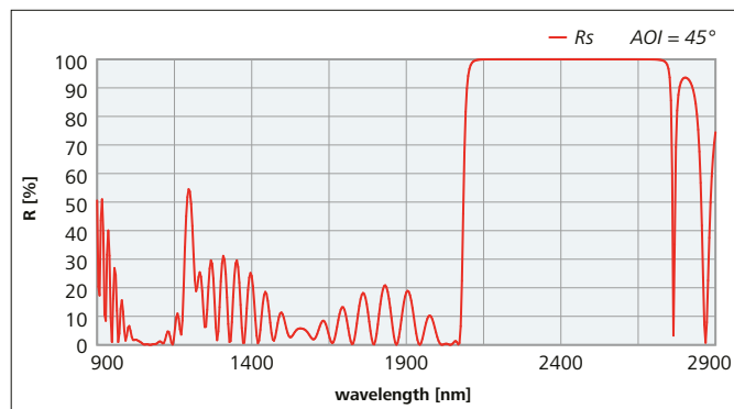
Figure 15: Reflectance spectrum of an edge filter for the idler and signal wavelength range with high transmittance for the pump wavelength: HRs(45^\circ, 2150 - 2700 \text{ nm}) > 99.9 \% + R_s(45^\circ, 2000 - 2070 \text{ nm}) < 10 \% + R_s(45^\circ, 1064 \text{ nm}) < 1 \%
