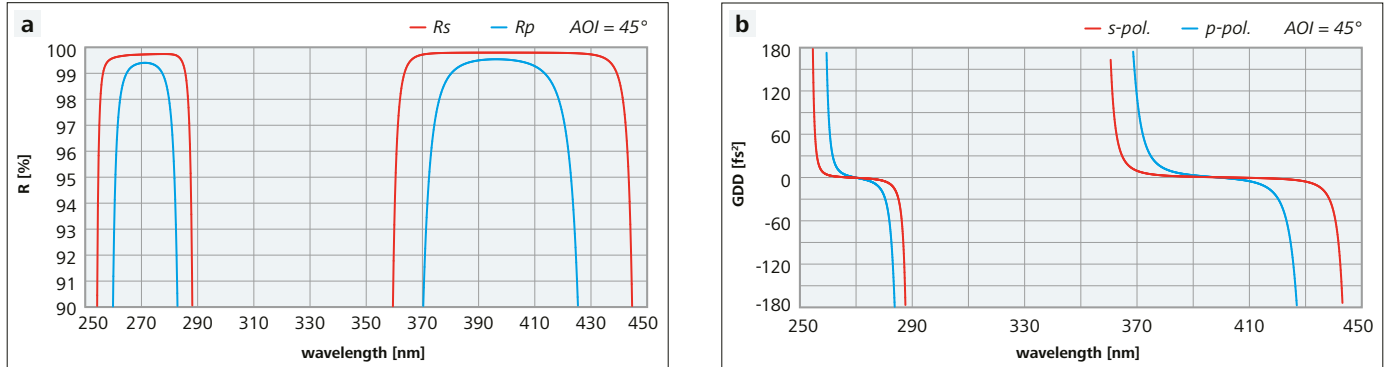
Figure 1: Reflectance and GDD spectra of a fs-optimized dual wavelength turning mirror for 270 nm and 405 nm
