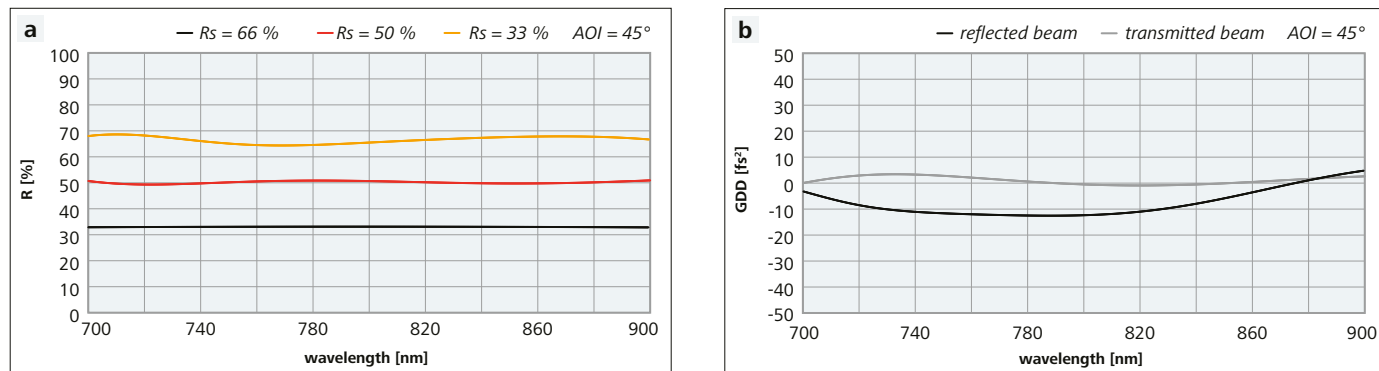
Figure 6: Reflectance and GDD spectra of beam splitters for s-polarized light
