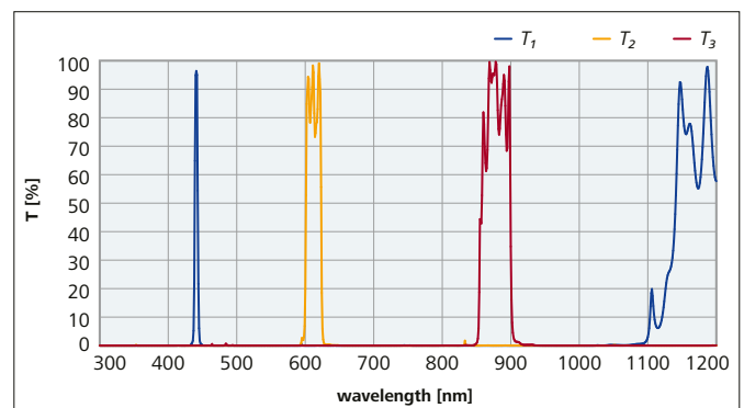
Figure 4: Calculated transmission for three different lateral positions of AOI = 0^\circ
