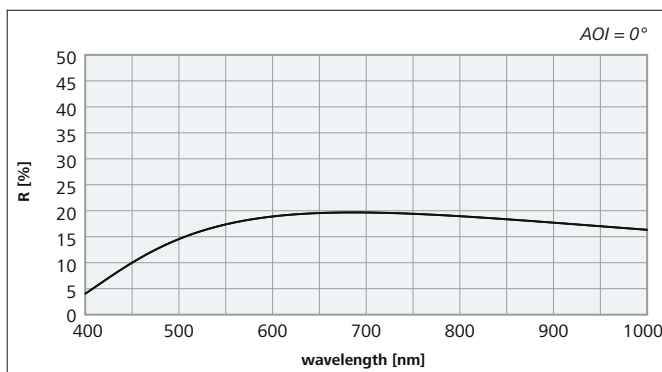
Figure 4: Reflectance spectrum of an output coupler for the ruby laser: PR (0°, 694 nm) = 20 % \pm 2 %
