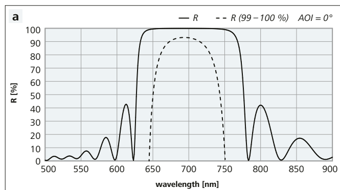
Figure 1: Reflectance spectra of cavity mirrors for:
