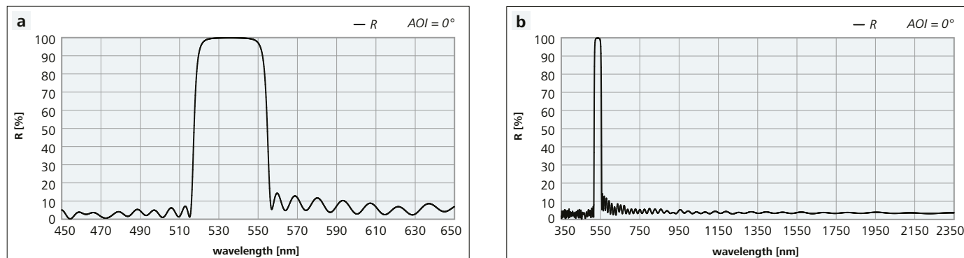
Figure 6: Reflectance spectrum of a narrowband reflectance filter for 550 nm
