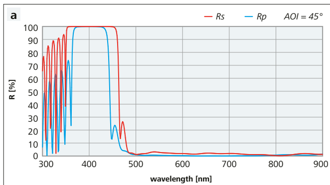
Figure 3: Reflectance and GDD spectra of a separator HRs,p (45°, 400 nm) > 99.9 % + Rs,p (45°, 800 nm) < 2 % a) Reflectance vs. wavelength b) GDD vs. wavelength
