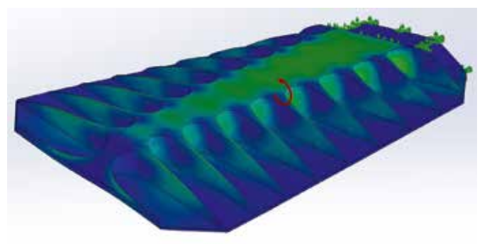
Figure 24: FEM simulation of mechanical deformation (blue = “stress-free”, green = “stresses due to deformation”, red arrow = “torsional direction”). The stresses in the component are homogeneously distributed, there are no stress peaks. This ensures optimum performance.
