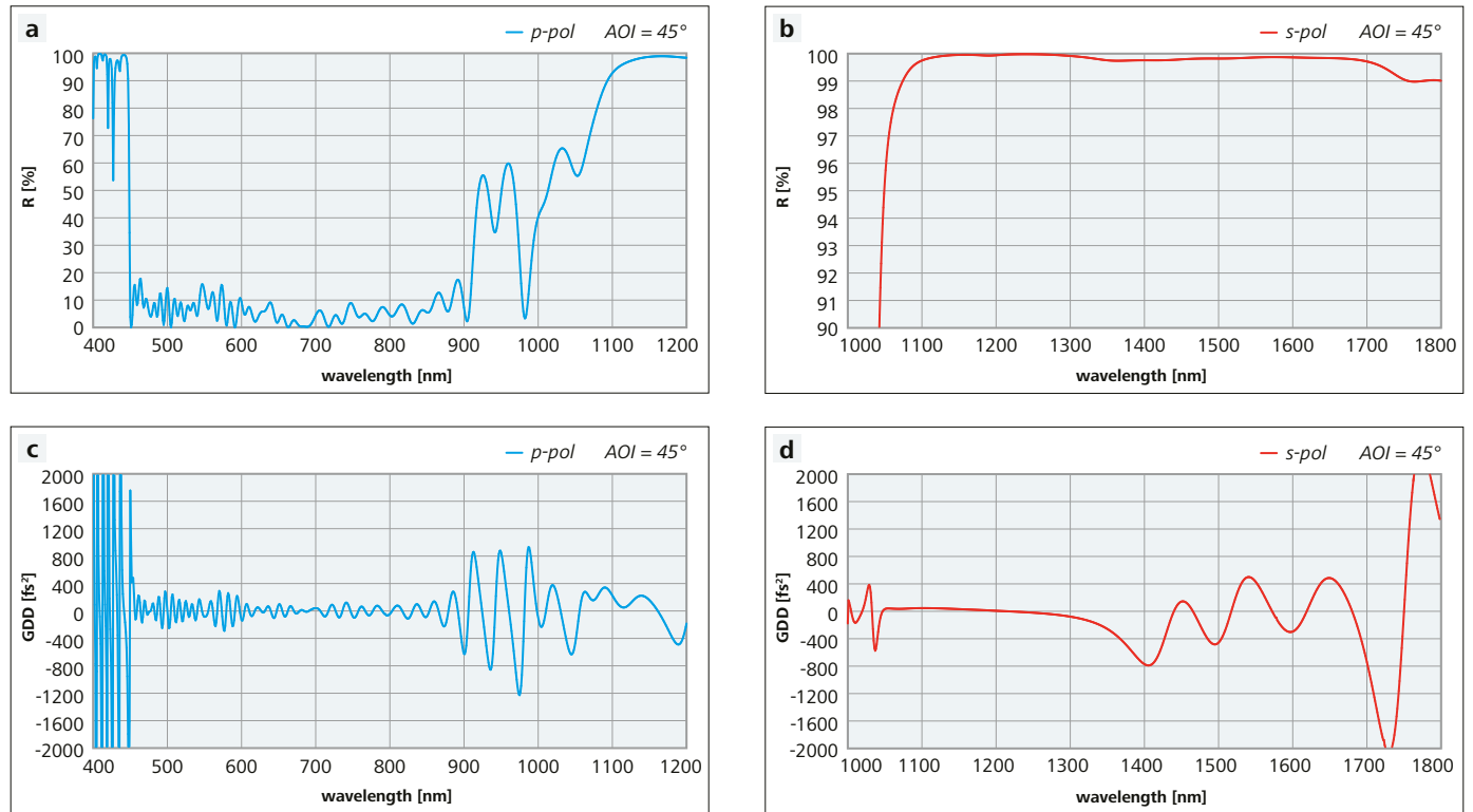
Figure 6: Reflectance and GDD spectra of a beam combiner:
