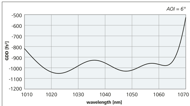
Figure 7: Calculated GDD spectrum of a GTI mirror: GDD-R (6°, 1020 – 1060 nm) \approx -1000 \pm 200 \text{ fs}^2
