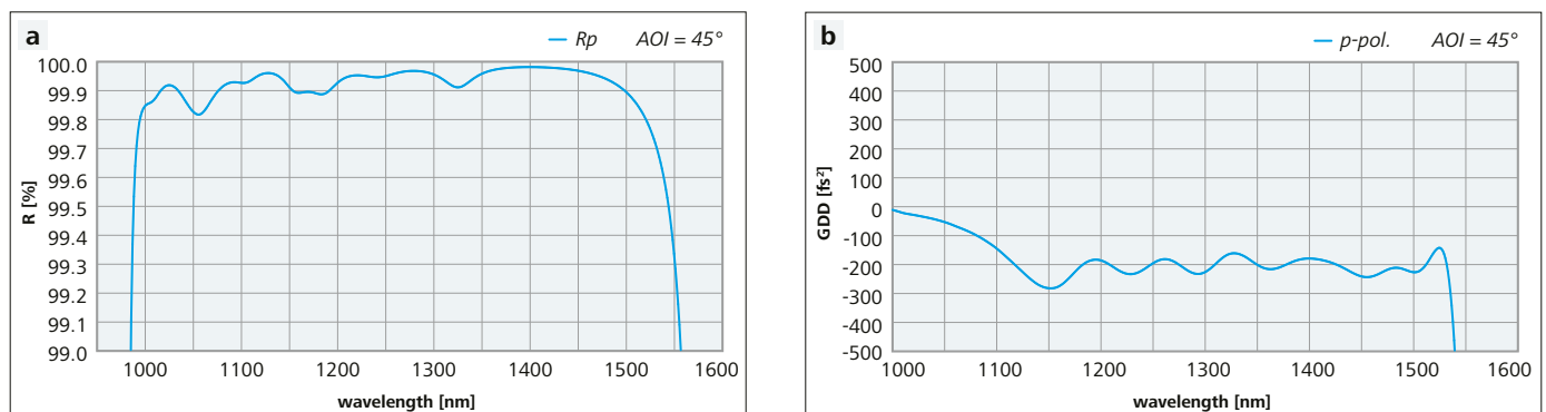
Figure 5: Reflectance and GDD spectra of a broadband negative dispersion turning mirror
