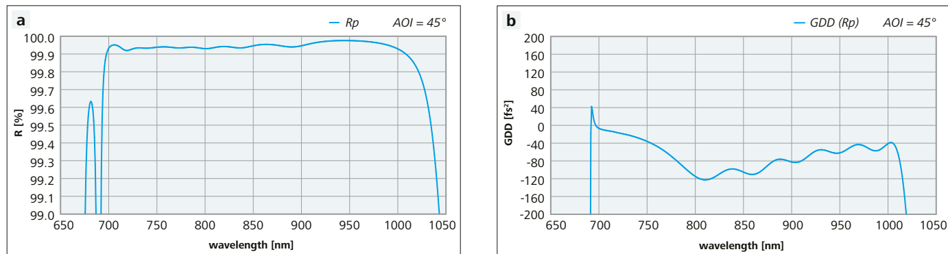
Figure 3: Reflectance and GDD spectra of a broadband turning mirror for p-polarized light
