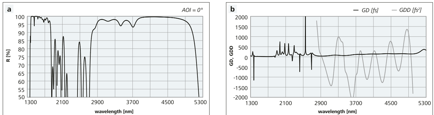
Figure 2: Reflectance, GD and GDD spectra of a dual HR mirror for the signal and idler wavelengths:
