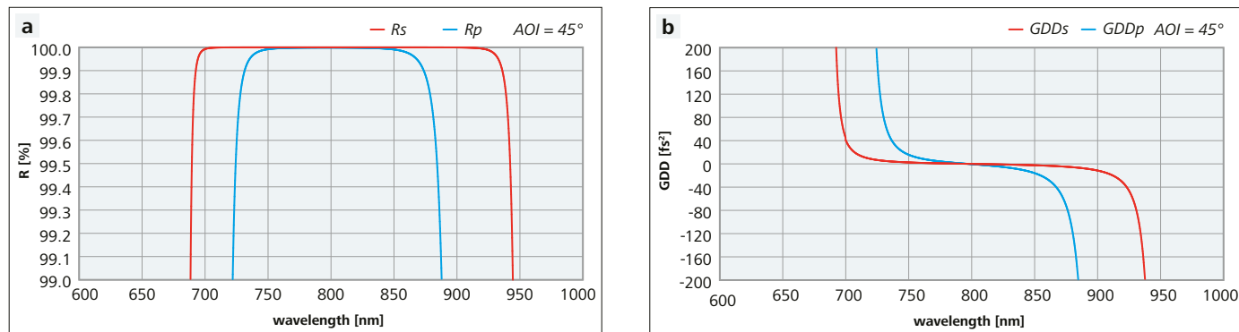
Figure 3: Reflectance and GDD spectra for a standard low dispersion turning mirror (bandwidth R_u (45°) > 99.9 % \approx 160 nm)
