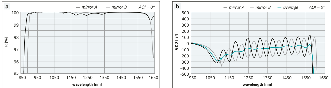
Figure 4: Reflectance and GDD spectra of a broadband negative dispersion mirror pair; single mirrors with R > 99.7\% (mirror A) and R > 99.85\% (mirror B)
