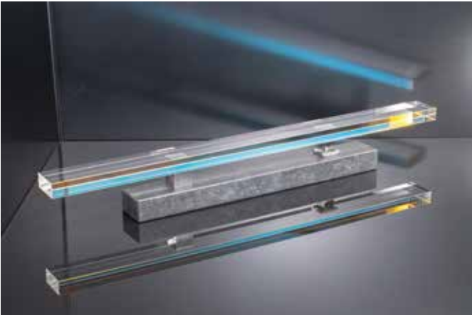
Figure 1: Large high-accuracy reference mirror mounted on a mechanically stiff bracket on one side
