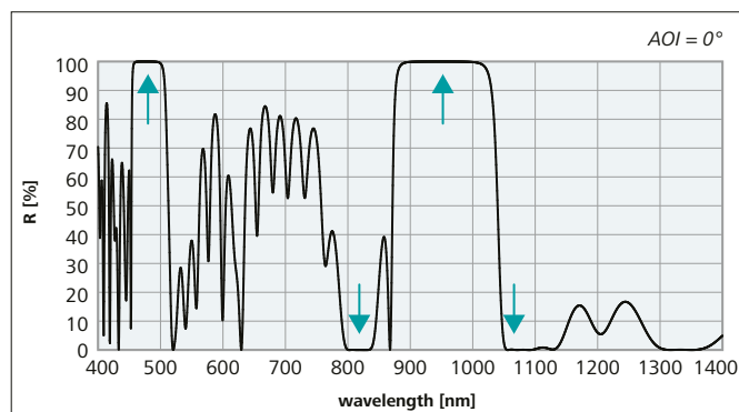
Figure 1: Reflectance spectrum of a dual wavelength mirror for a weak laser line and its second harmonic with high transmittance for the pump wavelength and the strongest laser line: HR (0°, 473 nm) > 99.85 % + HR (0°, 946 nm) > 99.95 % + R (0°, 808 nm) < 2 % + R (0°, 1064 nm) < 5 %
