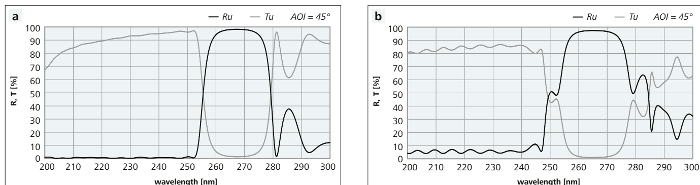
Figure 5: Reflectance spectra of separators for the fourth and fifth harmonics: HRu (45°, 266 nm) > 98 % + Ru (45°, 213 nm) < 10 % for unpolarized light
