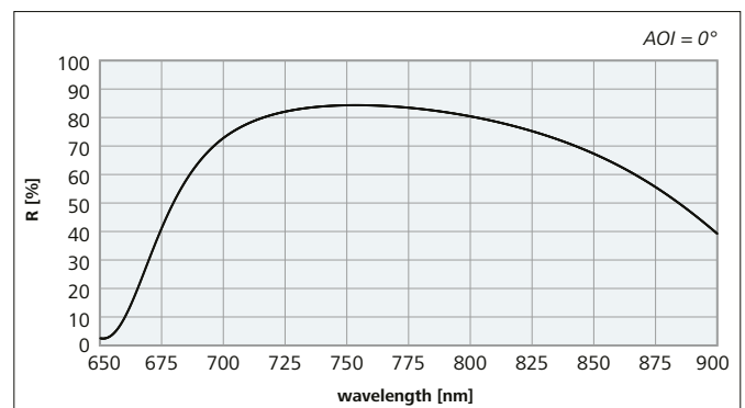
Figure 5: Reflectance spectrum of an output coupler for the alexandrite laser: PR (0°, 755 nm) = 85 % \pm 2 %
