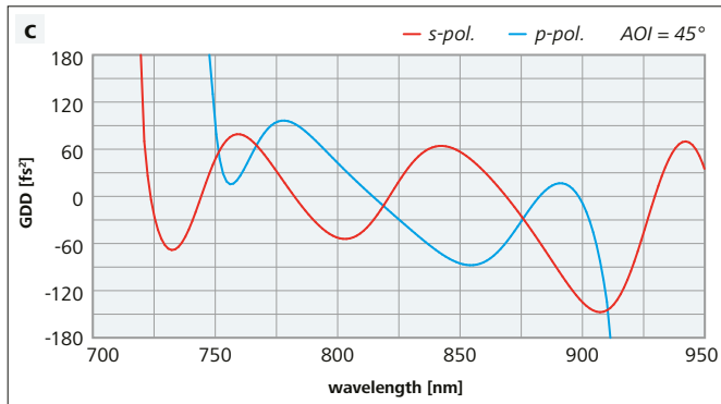
Figure 2: Reflectance and GDD spectra of a fs-optimized dual wavelength turning mirror for 400 nm + 800 nm at AOI = 45° a) Reflectance vs. wavelength b) GDD vs. wavelength (second harmonic) c) GDD vs. wavelength (fundamental)
