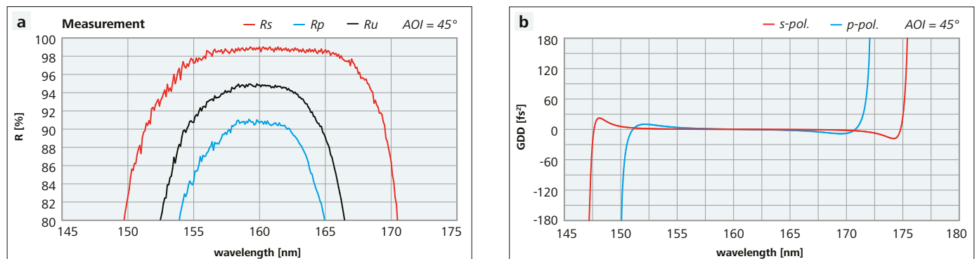
Figure 2: Reflectance and GDD spectra of a turning mirror for 160 nm (AOI = 45°) a) Reflectance vs. wavelength (measured) b) GDD vs. wavelength (calculated)
