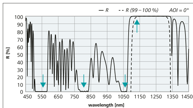
Figure 2: Reflectance spectrum of a dichroic mirror with high transmittance for the pump wavelength which also suppresses the 1064 nm line: HR (0°, 1123 nm) > 99.9 % + R (0°, 561 nm) < 2 % + R (0°, 808 nm) < 10 % + R (0°, 1064 nm) < 50 %
