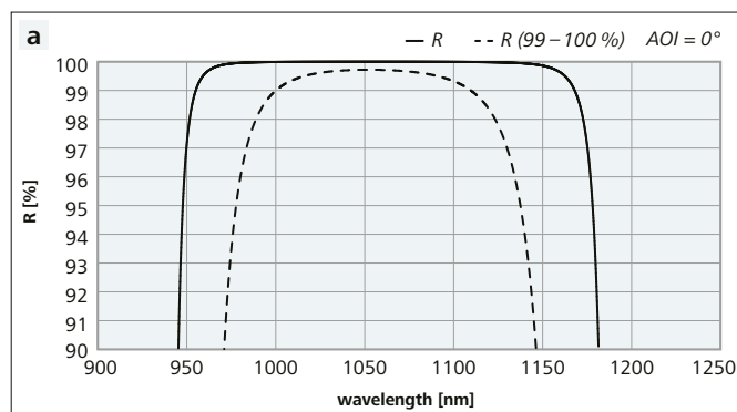
Figure 1: Reflectance spectra of HR mirrors for 1030 nm
