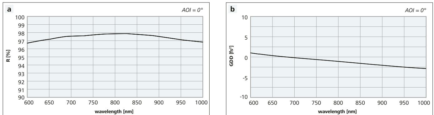
Figure 1: Reflectance and GDD spectra of a silver mirror optimized for use with ultrafast-lasers in the wavelength range 600 – 1000 nm (AOI = 0°)
