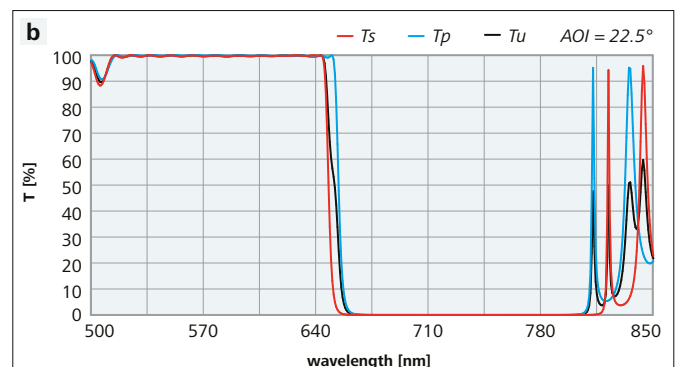
Figure 5: Transmittance spectra of a steep edge short-wavelength pass filter for use as a combiner for laser diodes at 635 nm and 670 nm HRu ( 22.5^\circ , 670 nm) > 99.9 % + Ru ( 22.5^\circ , 635 nm) < 2 %, rear side AR coated)
