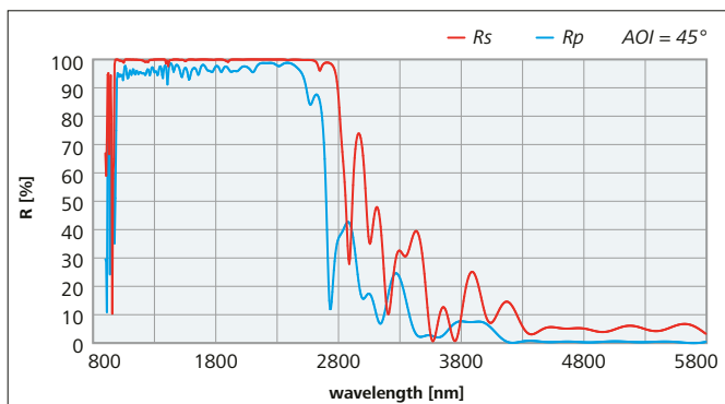
Figure 14: Reflectance spectrum of an ultra broadband separator for signal and idler wavelengths: HRu (45°, 1000 – 2500 nm) > 98 % + Ru (45°, 4400 – 5000 nm) < 5 %
