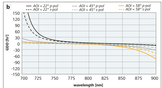
Figure 4: Reflectance and GDD spectra of a scanning mirror for ultrafast laser pulses from a Ti:Sapphire laser: HRu (22° – 58°, 750 – 850 nm) > 99.5 %, |GDD-Ru (22° – 58°, 750 – 850 nm)| < 20 fs 2
