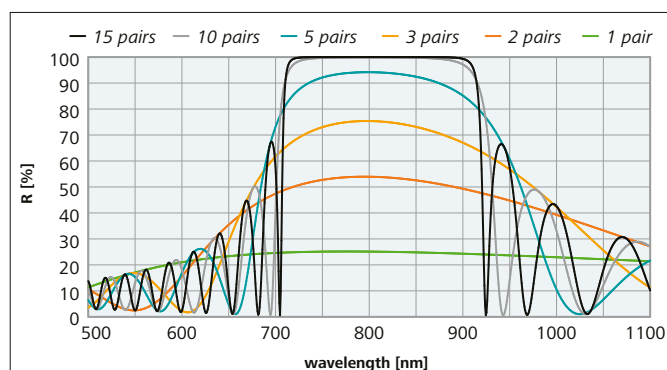
Figure 5: Calculated reflectance of quarter-wave stacks consisting of 1, 2, 3, 5, 10 and 15 layer pairs of \text{Ta}_2\text{O}_5/\text{SiO}_2 for 800 nm
