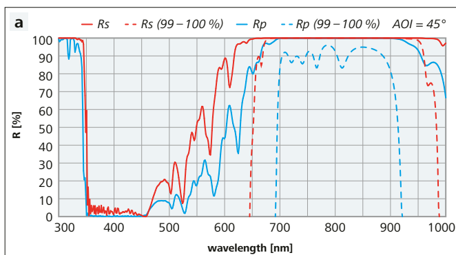
Figure 4: Reflectance and GDD spectra of a separator HRp (45°, 800 nm) > 99.9 % + Rp (45°, 400 nm) < 2 % + Rs (45°, 400 nm) < 10 % a) Reflectance vs. wavelength b) GDD vs. wavelength
