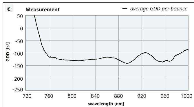
Figure 9: Reflectance and GDD spectra of a high dispersion mirror pair with a bandwidth of 200 nm and an average GDD of -120 \pm 40 \text{ fs}^2 per bounce in the 800 nm range
