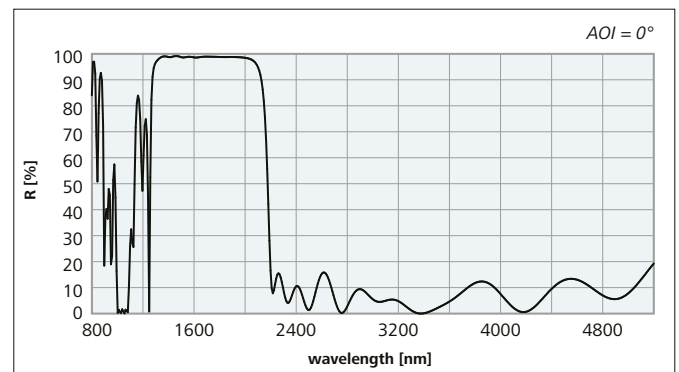
Figure 10: Reflectance spectrum of a special output coupler: PR (0°, 1350 – 2000 nm) = 98 % \pm 0.5 % + R (0°, 1000 – 1100 nm) < 3 % + R (0°, 2200 – 5000 nm) < 20 %
