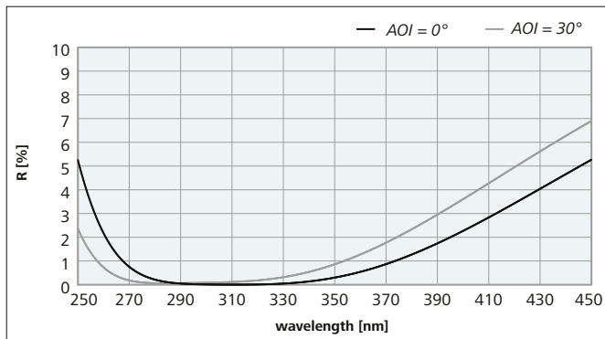
Figure 5: Reflectance spectra of an AR coating for 308 nm and \text{AOI} = 0^\circ - 30^\circ
