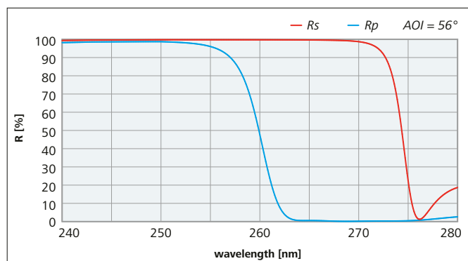
Figure 6: Reflectance spectrum of a thin film polarizer for 266 nm:
