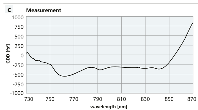
Figure 8: Reflectance and GDD spectra of a high dispersion mirror with a bandwidth of 120 nm and a GDD of -450 \pm 100 \text{ fs}^2 in the 800 nm range
