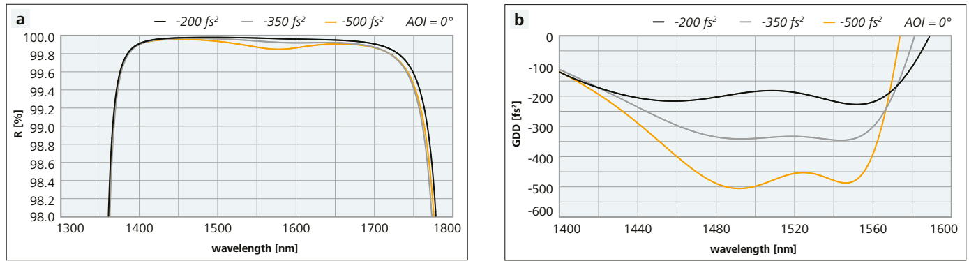
Figure 3: Reflectance and GDD spectra of GTI mirrors for 1500 nm with different GDD values
