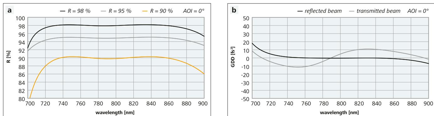
Figure 4: Reflectance and GDD spectra of output couplers with a bandwidth of 120 nm
