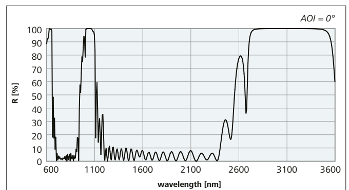
Figure 20: Reflectance spectrum of a double reflector with two regions of high transmittance on lithium niobate: HR(0^\circ, 1010 - 1075 + 2750 - 3450 \text{ nm}) > 99.8 \% + R(0^\circ, 700 - 900 + 1200 - 2400 \text{ nm}) < 10 \%
