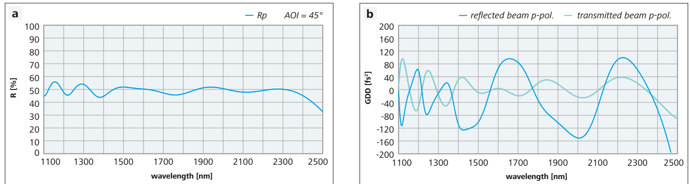
Figure 8: Reflectance and GDD spectra of a broadband beam splitter for p-polarized signal and idler radiation: PRp (45°, 1100 – 2400 nm) = 50 % \pm 5 %
