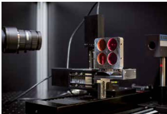
Figure 12: Sample stage of the LIDT measurement set-up
