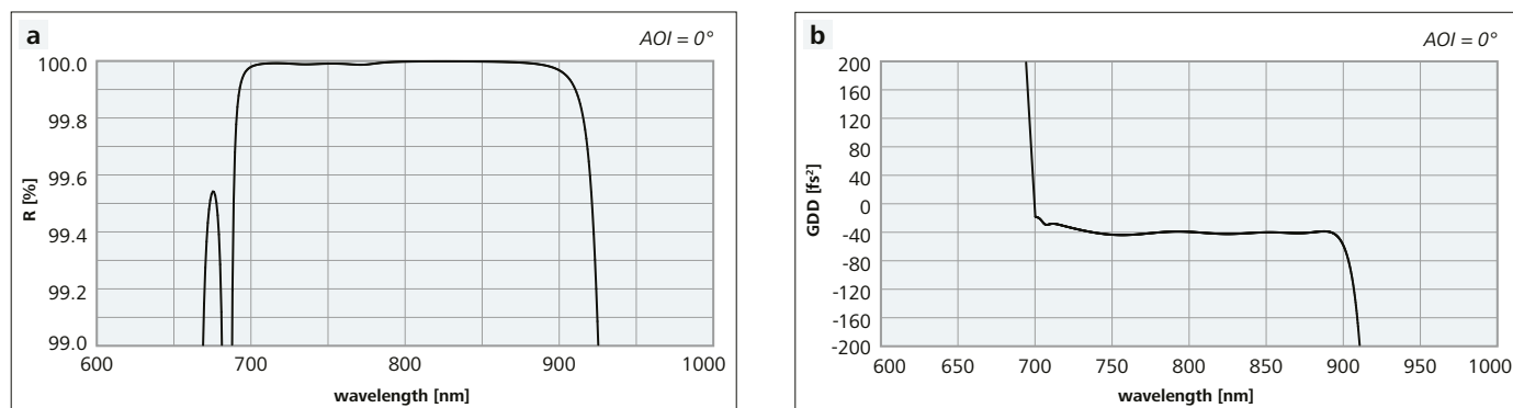
Figure 7: Reflectance and GDD spectra of a negative dispersion mirror with a bandwidth of 150 nm
