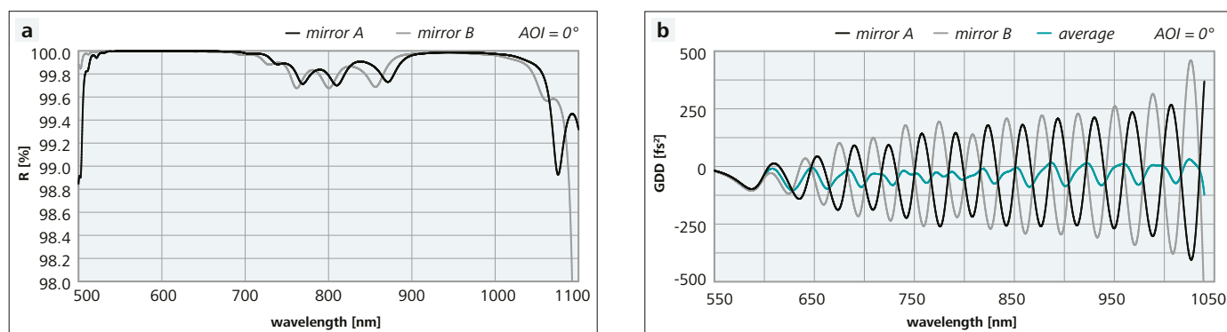
Figure 1: Reflection and GDD spectra of a pair of ultra-broadband negative-dispersion laser mirrors
