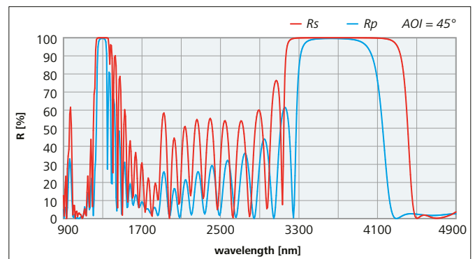
Figure 16: Reflectance spectrum of a broadband edge filter for the idler wavelength range with high transmittance for the pump wavelength: HRs(45^\circ, 3300 - 4200 \text{ nm}) > 99.9 \% + R_s(45^\circ, 4500 - 4900 \text{ nm}) < 6 \% + R_{s,p}(45^\circ, 1064 \text{ nm}) < 5 \%
