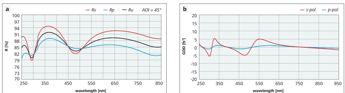
Figure 2: Reflectance and GDD spectra of an aluminum mirror optimized for R > 85\% at 266 nm, 400 nm and 800 nm (AOI = 45°)
