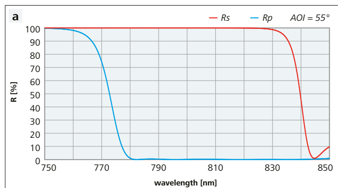
Figure 10: Reflectance and GDD spectra of a standard TFP (AOI = 55° to use the Brewster's angle for the transmitted p-polarized light)
