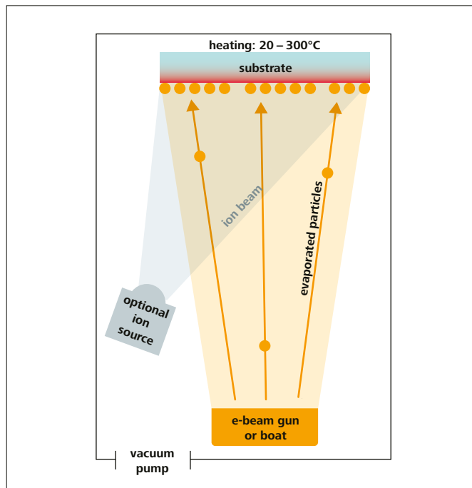
Figure 2: Schematic of an evaporation system
