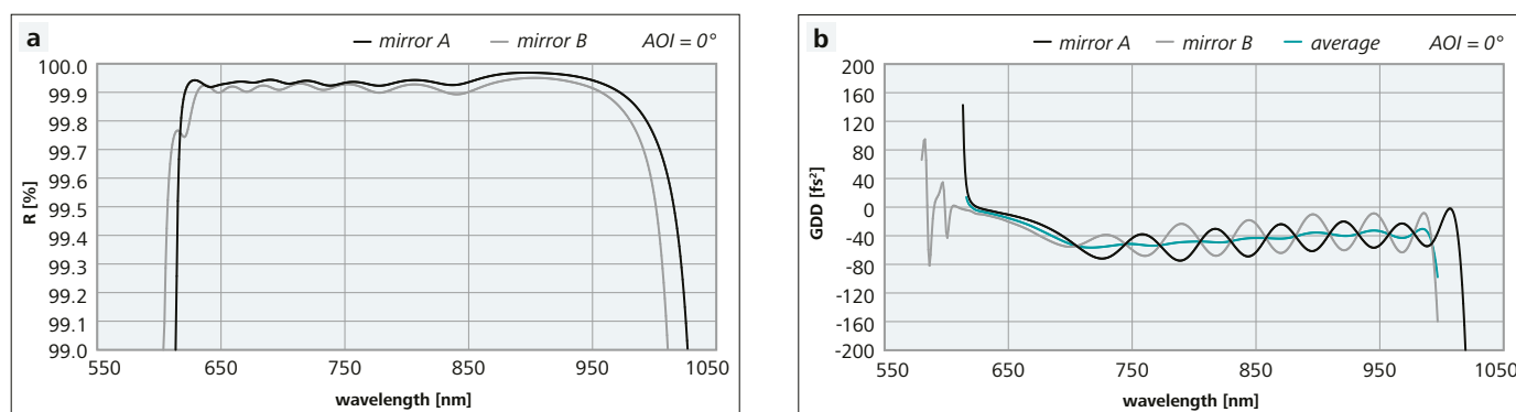
Figure 1: Reflectance and GDD spectra of a negative dispersion laser mirror pair
