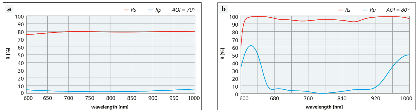
Figure 3: Broadband TFPs for the wavelength range of the Ti:Sapphire laser with different bandwidths and different polarization ratios, working at AOI = 70° and AOI = 80°
