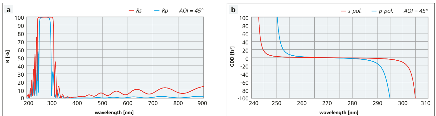
Figure 3: Reflectance and GDD spectra of a standard separator reflecting the third harmonic and transmitting the second harmonic and the fundamental
