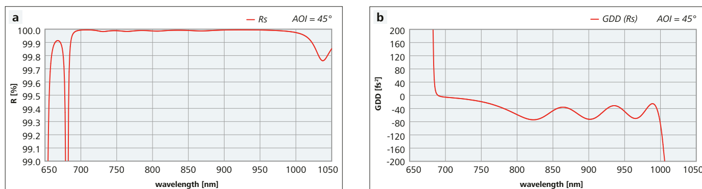
Figure 2: Reflectance and GDD spectra of a broadband turning mirror for s-polarized light
