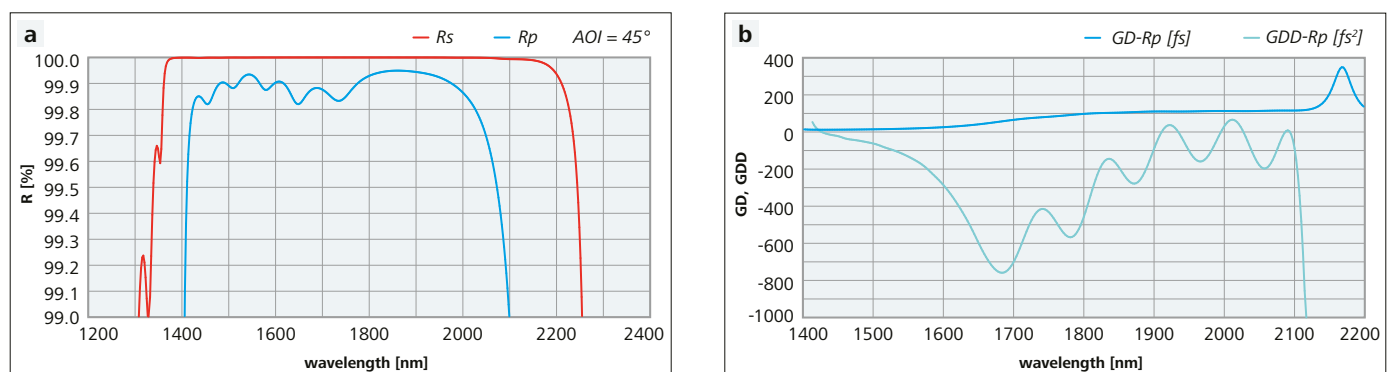
Figure 11: Reflectance, GD and GDD spectra of a turning mirror HRp (45°, 1450 – 2000 nm) > 99.8 %
