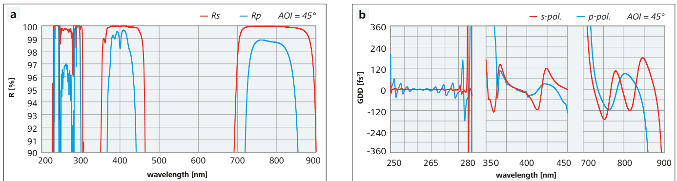
Figure 2: Reflectance and GDD spectra of a fs-optimized turning mirror for the 266 nm, 400 nm and 800 nm wavelength regions
