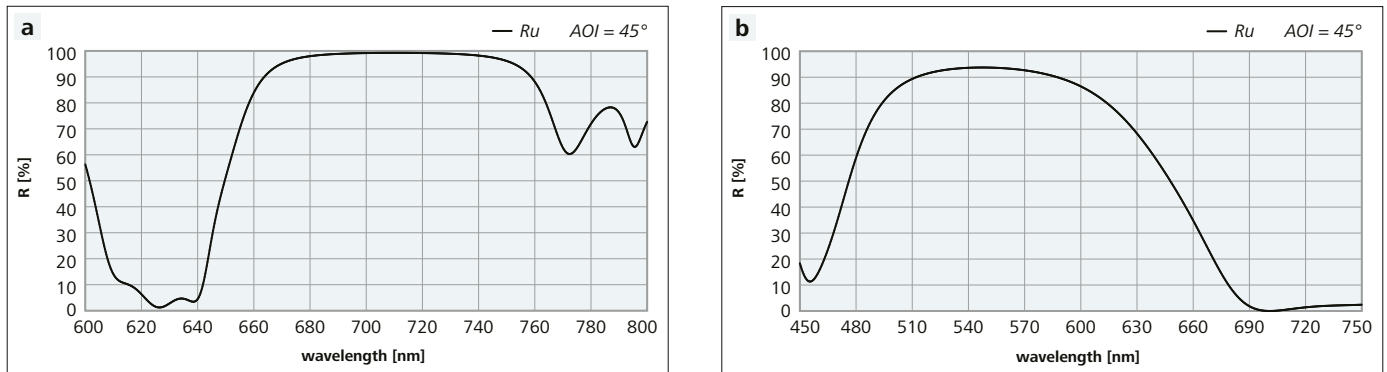
Figure 3: Reflectance spectra of special beam combiners for 694 nm and 633 nm:
