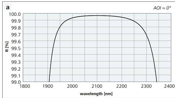
Figure 1: Reflectance spectra of cavity mirrors:
